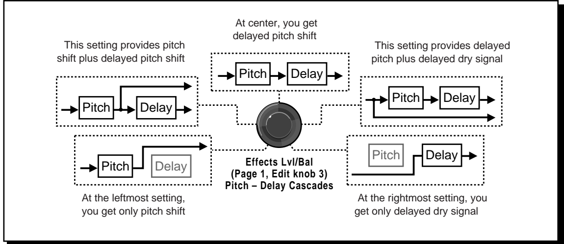
Behavior of Effects Lvl/Bal in the cascade programs. Several points from the knob's continuous range are illustrated here, using Pitch-Delay as an example.
